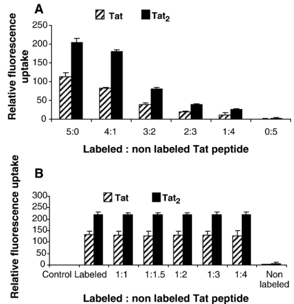
Fig. 7. Competition experiments suggested free, passive nuclear transport of Tat peptides. (A) Total peptide concentration was kept constant (5 \mu M) and the ratio of labeled and non-labeled peptide was varied. (B) concentration of the labeled peptide was fixed (5 \mu M) and concentration of the non-labeled peptide was increased maximum up to 20 \mu M.
