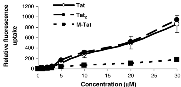
Fig. 3. Fluorimetric studies of the effect of concentration on the permeation potential of fluorescently labeled Tat peptides; Tat, Tat 2 and M-Tat in triticale mesophyll protoplasts.
